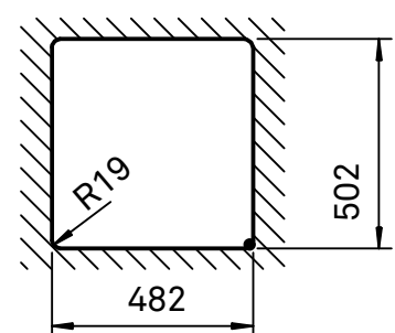
Installation: flush-mount
